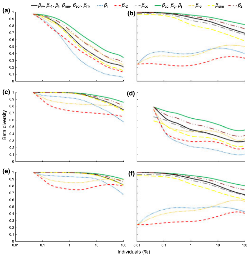
Figure 4 Beta diversity accumulation curves for the sampling at a local scale. The three methods employed at each of two studied sites are compared. For spiders in Gerês: (a) beating × sweeping; (c) sweeping × pitfall traps; (e) beating × pitfall traps. For arthropods in Pico: (b) beating × ethylene glycol traps; (d) ethylene glycol traps × Turquin traps; (f) beating × Turquin traps. The ordinate refers to the mean value of the given beta diversity index over 10,000 replicate simulations.
